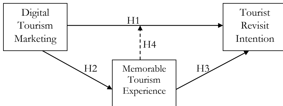
Figure 1. Framework Research
